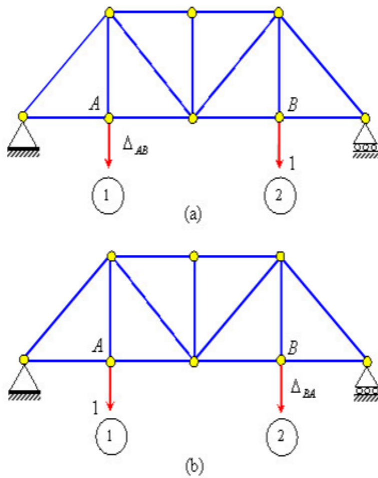
Figure 4.31 Illustration of Maxwell-Betti Law (directions 1 and 2 are shown by circle)
